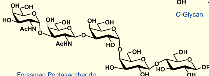
Forssman Pentasaccharide
