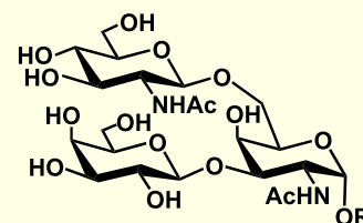
O-Glycan
