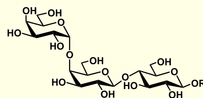
Globotriose
